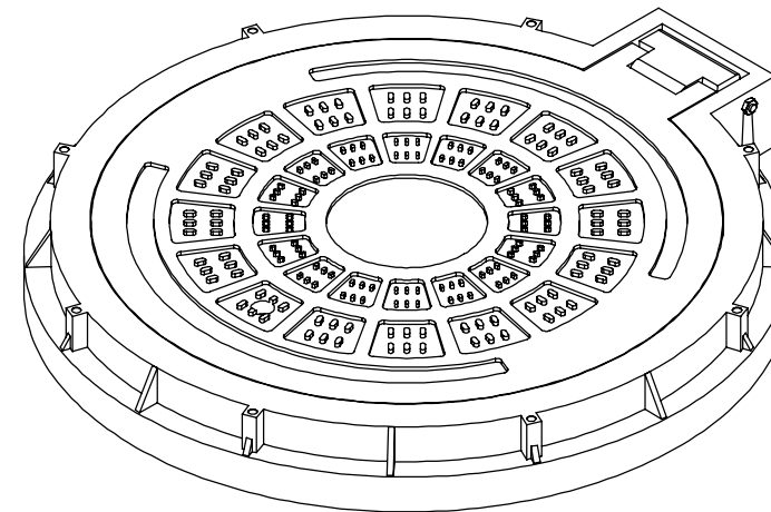
ISOMETRIC VIEW
